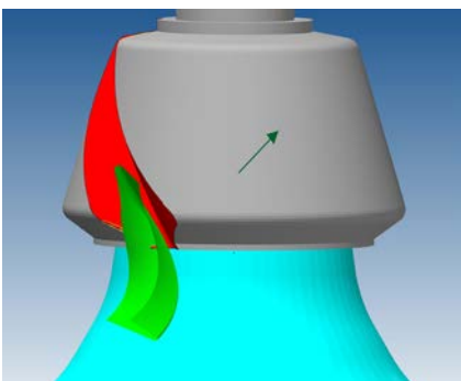
Fig. 9: Comparison of the two possible coupling situations for the same deburring task
