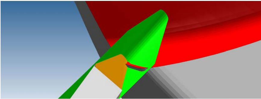
Fig. 6: Action of the deburring blade cutting edge at the tooth root and final shape of the deburring edge after a single cut
