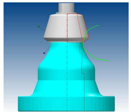
Fig. 5: Envelope contour of a clamping device and component (red); collision range of all deburring positions (green)
