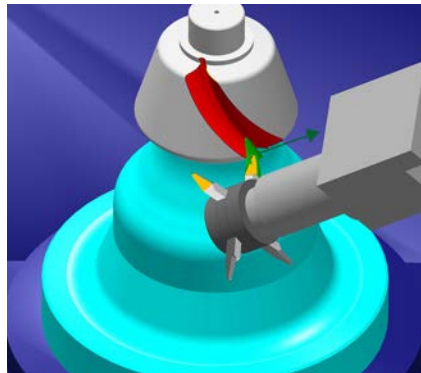
Fig. 2: 3D view of all components involved in the deburring task
