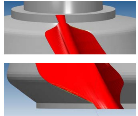
Fig. 3: Edges to be deburred, resulting from the cutting area between the component envelope and the component gap
